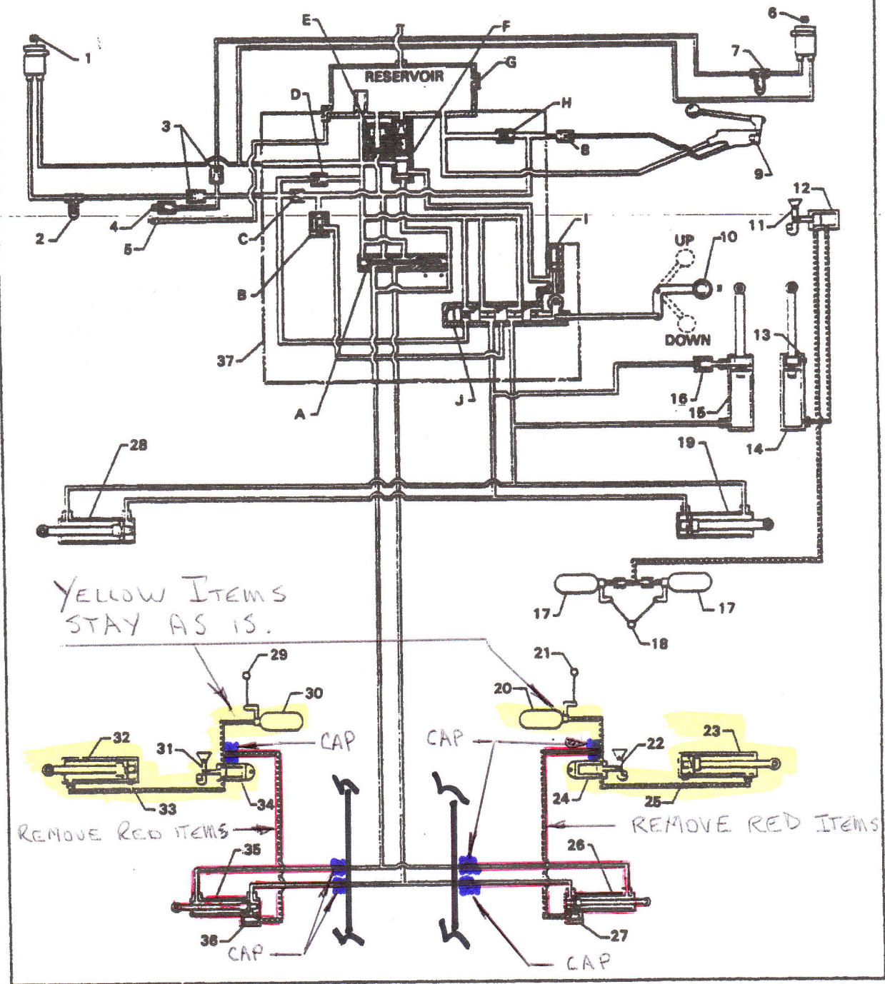
Figure 7-9c. Landing Gear Actuating System (PA-31T2)
